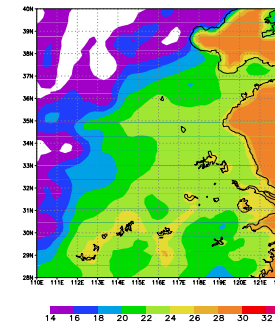
JSM-SiBUC (REANAL v1.5) 1998/07/02/06
