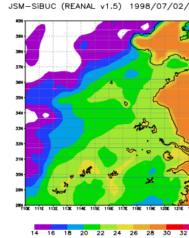
JSM-SiBUC (REANAL v1.5) 1998/07/02/09
