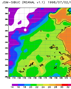
JSM-SiBUC (REANAL v1.1) 1998/07/02/09
