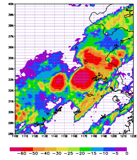
GMS-5 IR1 (degC) 1998/07/02/06
