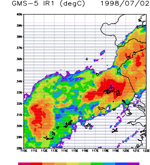
GMS-5 IR1 (degC) 1998/07/02/09
