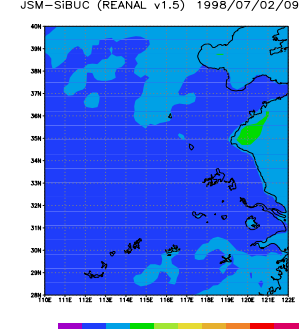
JSM-SiBUC (REANAL v1.5) 1998/07/02/09
