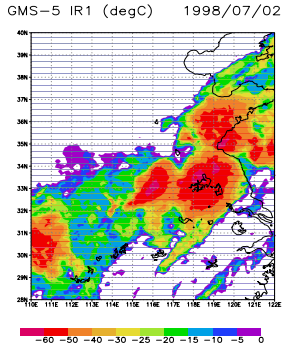
GMS-5 IR1 (degC) 1998/07/02/09
