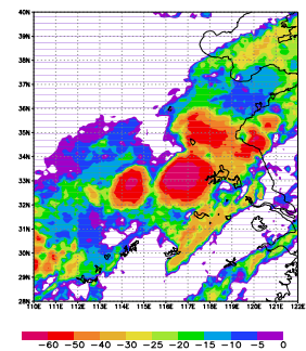
GMS-5 IR1 (degC) 1998/07/02/06
