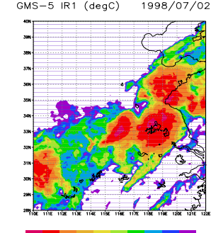
GMS-5 IR1 (degC) 1998/07/02/06
