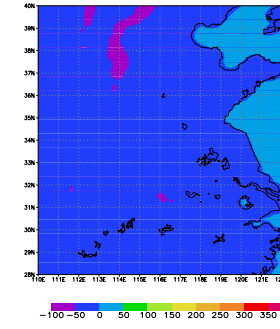
JSM-SiBUC (REANAL v1.1) 1998/07/02/06
