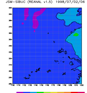
JSM-SiBUC (REANAL v1.5) 1998/07/02/06
